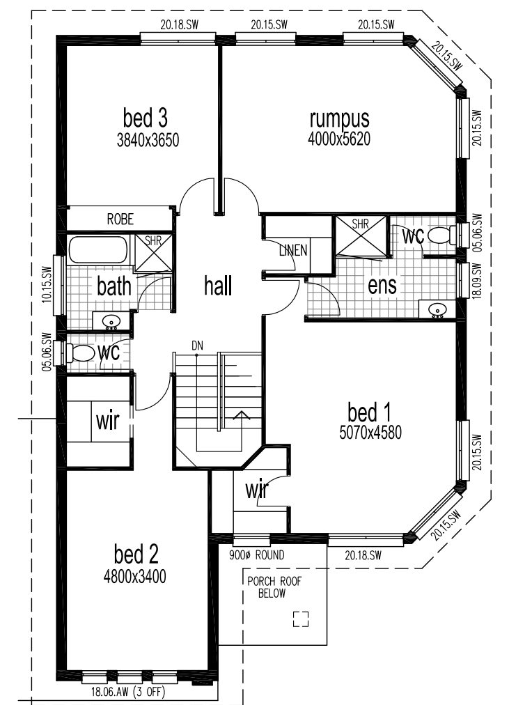
Upper Floor Plan "Option B" Rumpus to Rear and Bedroom One to Front
