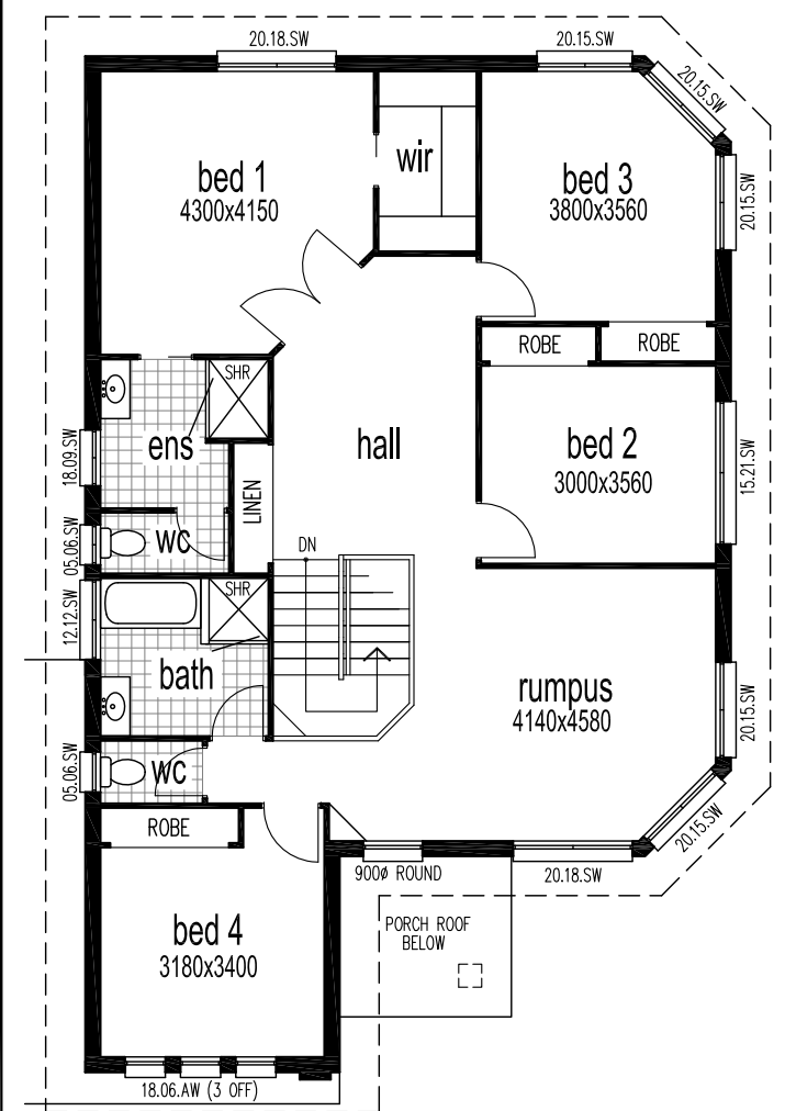
Upper Floor Plan "Option A" Rumpus to Front and Bedroom One to Rear
