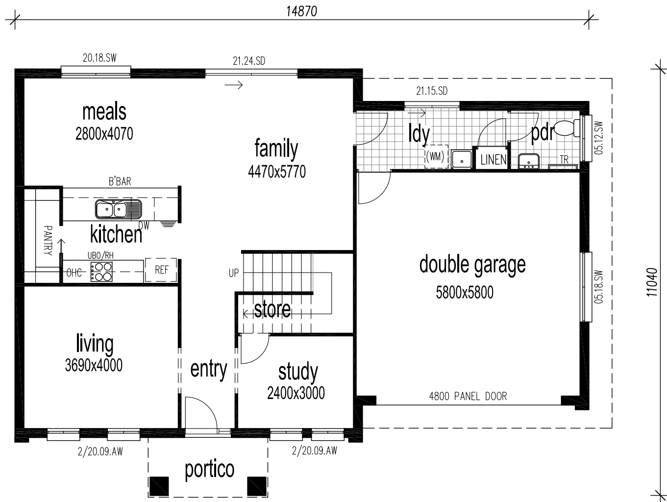
(Lower Floor Plan)
